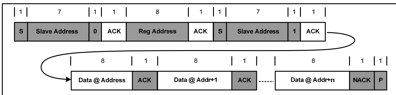
Figure 17: Multi-Read
