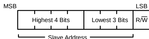
Figure 11: 7-Bit Address
