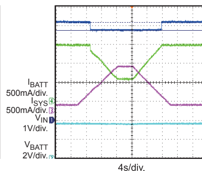
Input Voltage Clamp @ 4.6V
