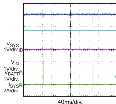
System Short Protection
