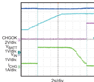
Battery Charge Curve
