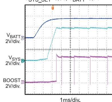
SYS Over Voltage Protection, Boost Mode
