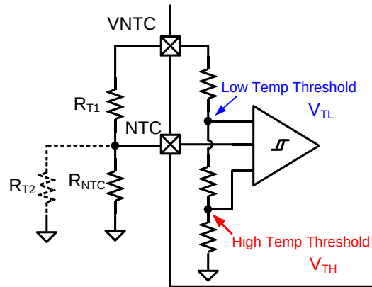
Figure 16: NTC Function Block
