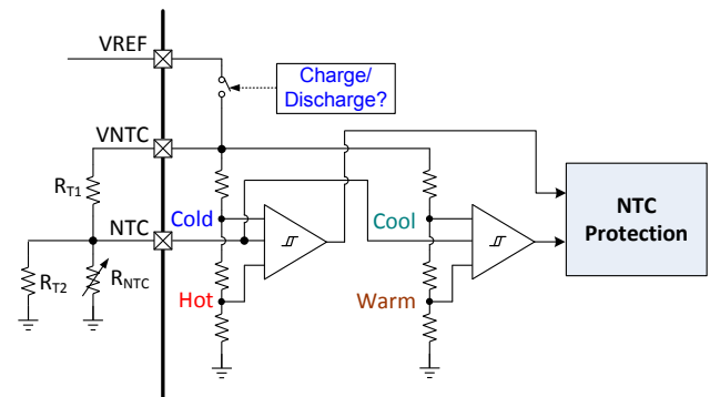
Figure 8: NTC Protection Circuit
