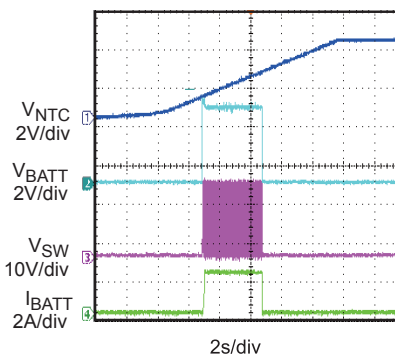
NTC Control
