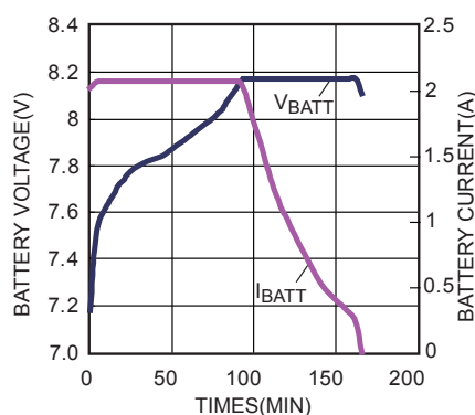
2-Cell Battery Charge Curve
