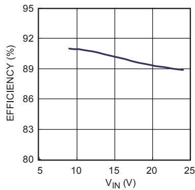
Efficiency vs. V IN 2-Cell, V BATT =7.4V, CC Load
