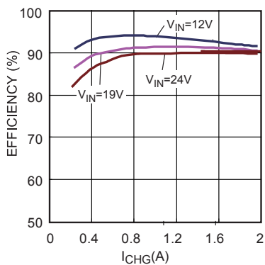
Efficiency vs. I CHG 2-Cell, V BATT =8.2V, CC Load
