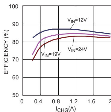
Efficiency vs. I CHG 1-Cell, V BATT =4.1V, CC Load
