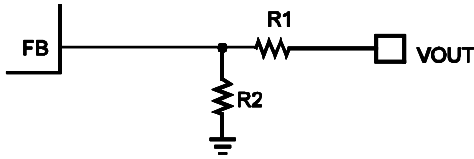
Figure 6: Feedback Network
