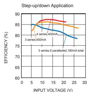
Efficiency vs. Input Voltage
