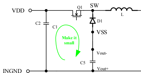
Figure 4—Buck-boost layout without VSS capacitor
