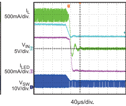
V_{IN} Shutdown
