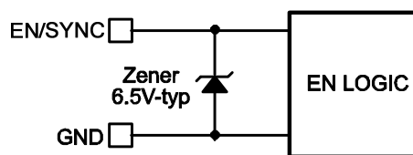
Figure 3: 6.5V Type Zener Diode
