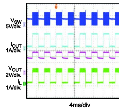
PWM Dimming
