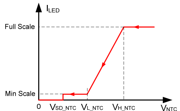
Figure 4: NTC Curve
