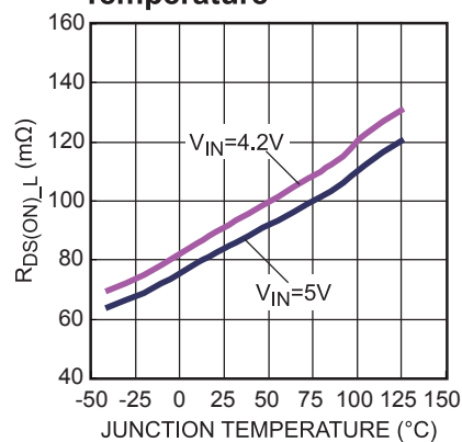
Low-Side Rectifier On Resistance vs. Junction Temperature
