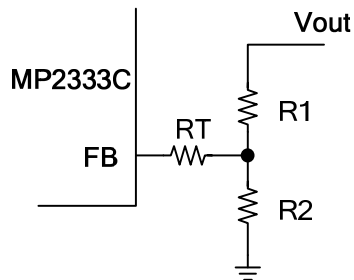
Figure 4: Feedback Network
