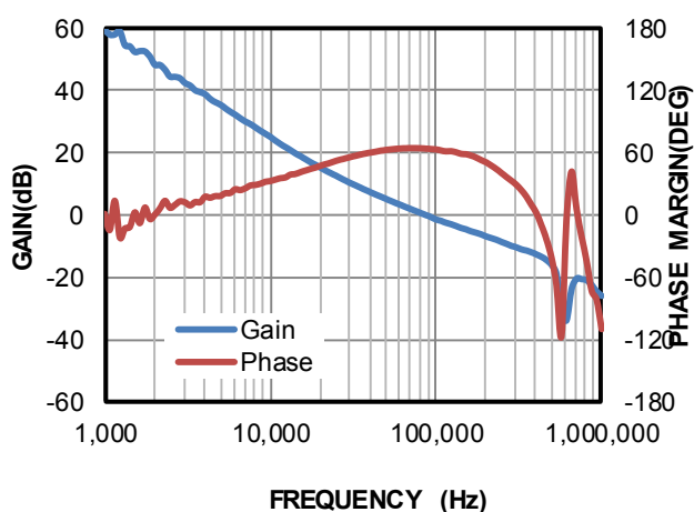
Bode Plot
