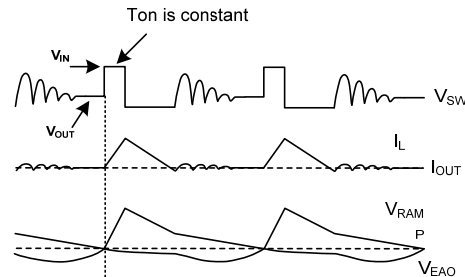
Figure 5: Light-Load Operation
