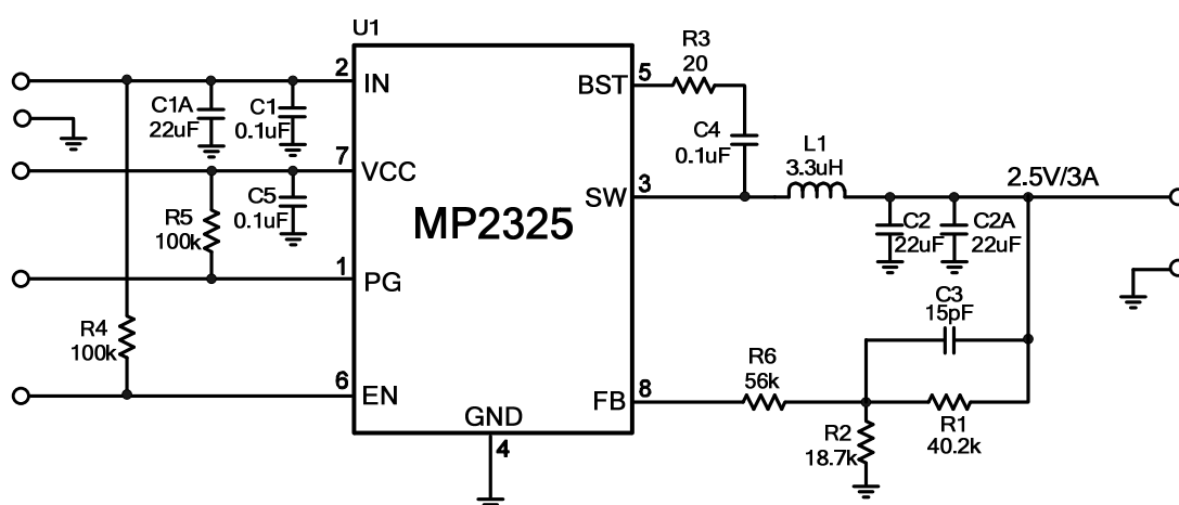
Figure 10: V_o=2.5V , I_o=3A
