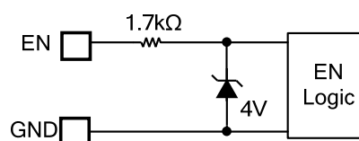
Figure 6: Zener Diode between EN and GND
