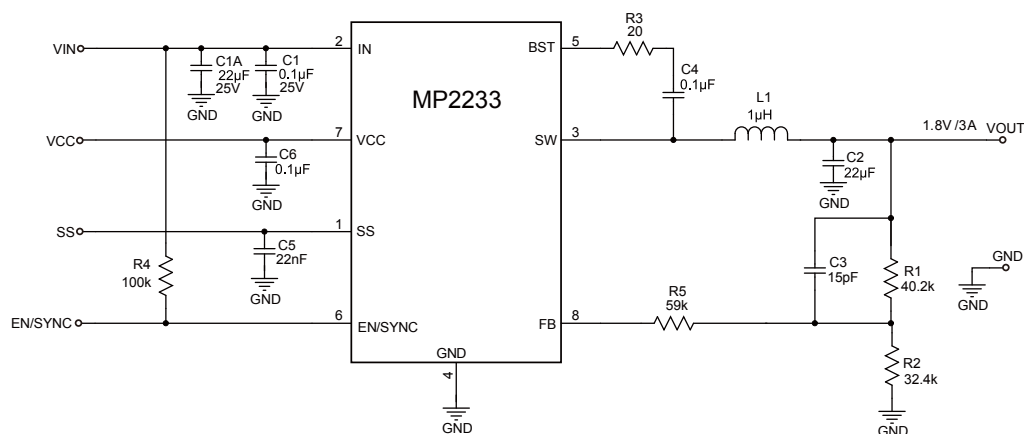
Figure 10: V_{IN} = 12V , 1.8V/3A Output
