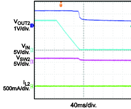
Shutdown through Input Voltage (CH2)
