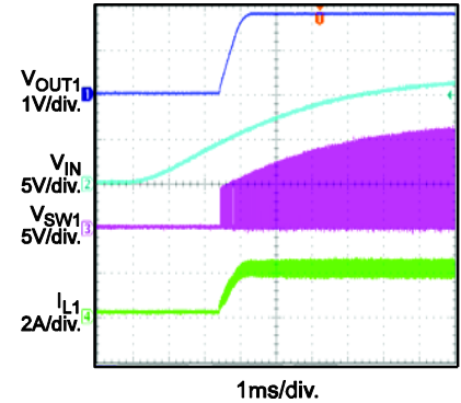
Startup through Input Voltage (CH1)
