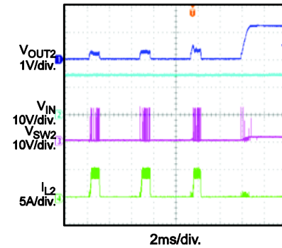
Shutdown through Input Voltage (Both CH1 and CH2 On)
