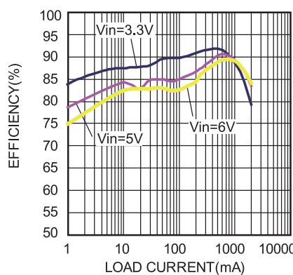
Efficiency
