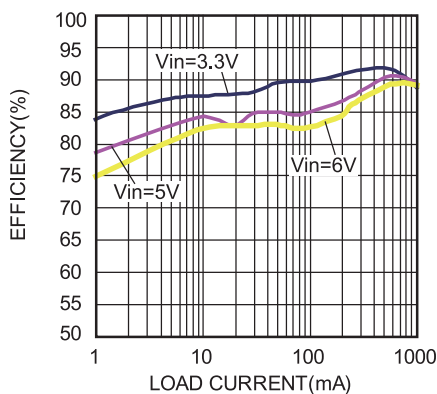
Efficiency
