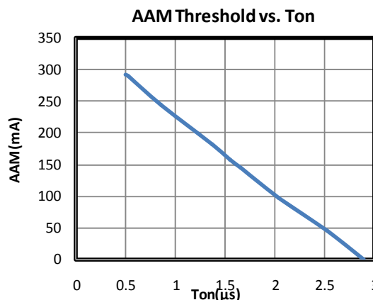
Figure 8: AAM Threshold Decreases as T_{ON} Increases
