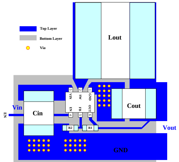
Figure 10: Recommended Layout for MP2151GTF
