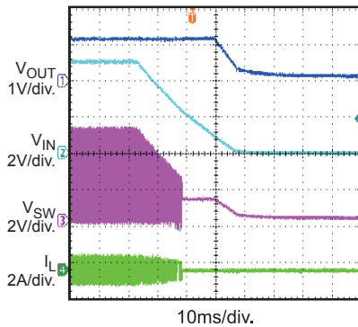
Power Off
