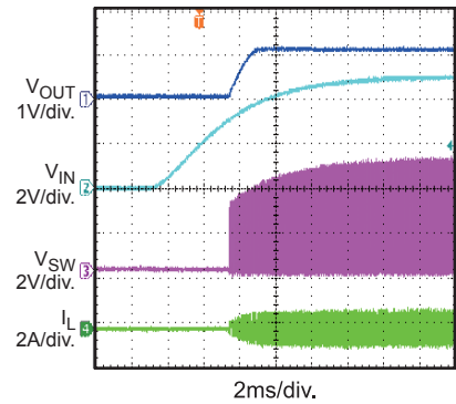
Power Up
