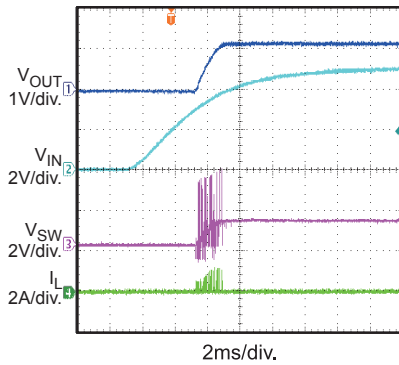
Power Up
