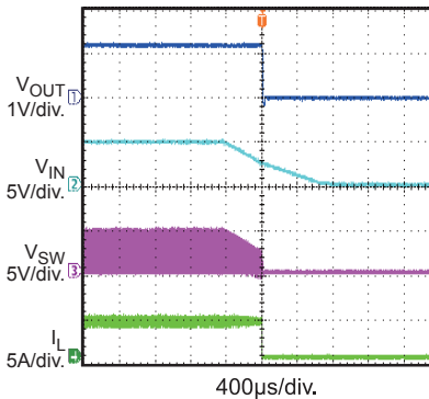
Power Off
