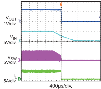
Power Off
