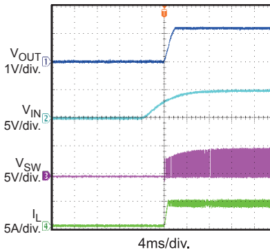
Power Up
