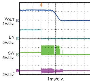
EN Shut Down without Load
