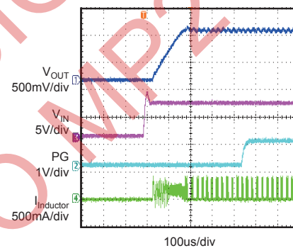
Power up for ASYN Mode I_{OUT} = 50mA , V_{OUT} = 0.9V
