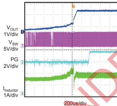
Short Recovery
