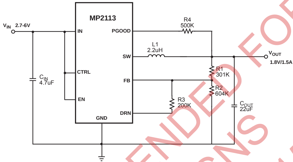
Figure 3-Typical Application Circuit
