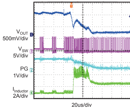
Output Short for ASYN Mode V_{OUT} = 0.9V , I_{OUT} = 50mA
