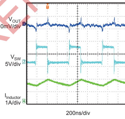
Output Ripple Voltage
