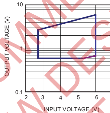
Operating Range
