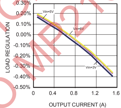
Load Regulation
