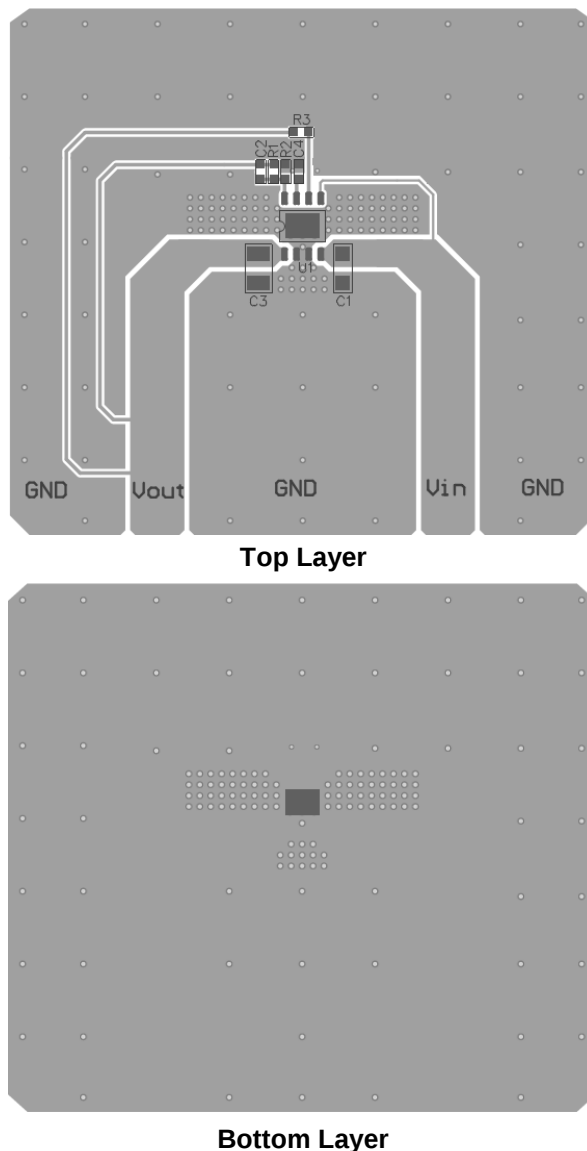
Figure 5. Recommended PCB Layout
