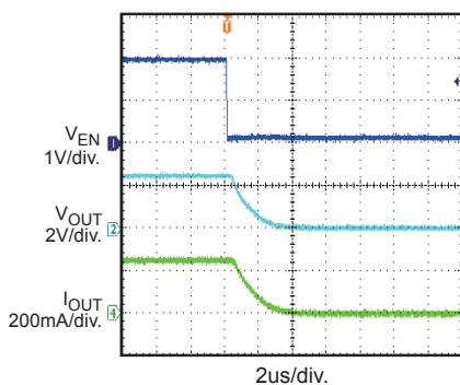
EN Shut Down with Resistive Load
