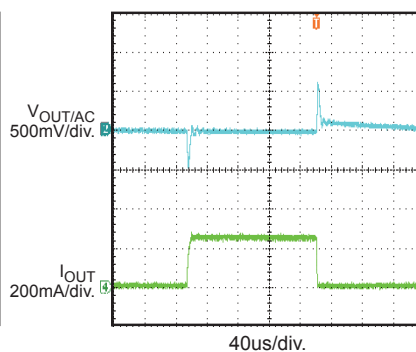
Load Transient with Resistive Load
