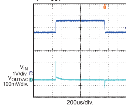
Line Transient with Resistive Load
