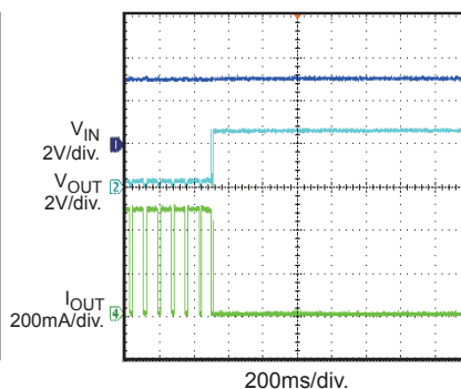
Over Current Protection Recovery
