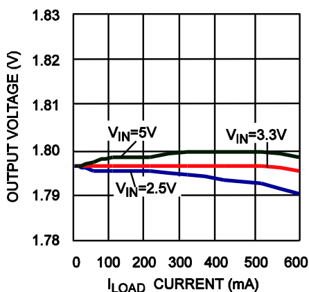
Load Regulation at -40°C
