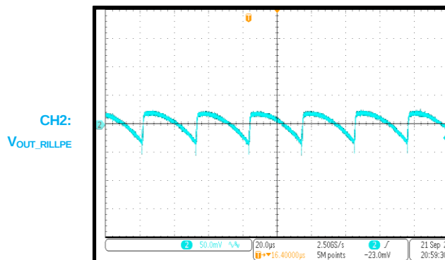
Output Ripple
