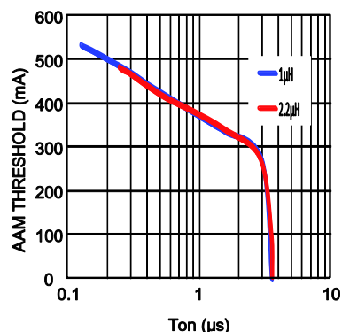
Figure 9: AAM Threshold Decreases as T_{ON} Increases
