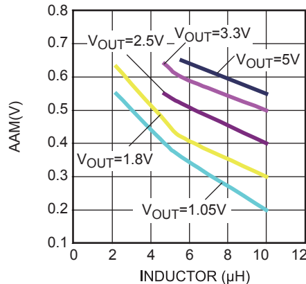
Figure 6: AAM Selection for Common Output Voltages ( V_{IN}=4.5V to 16V )
