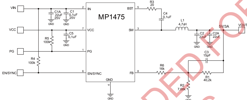
Figure 7: 12V IN , 5V/3A Output
