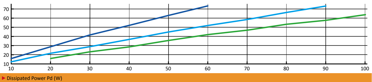
Heat sink to ambient temperature rise T_{hs-amb} (°C) vs Dissipated Power Pd (W)
