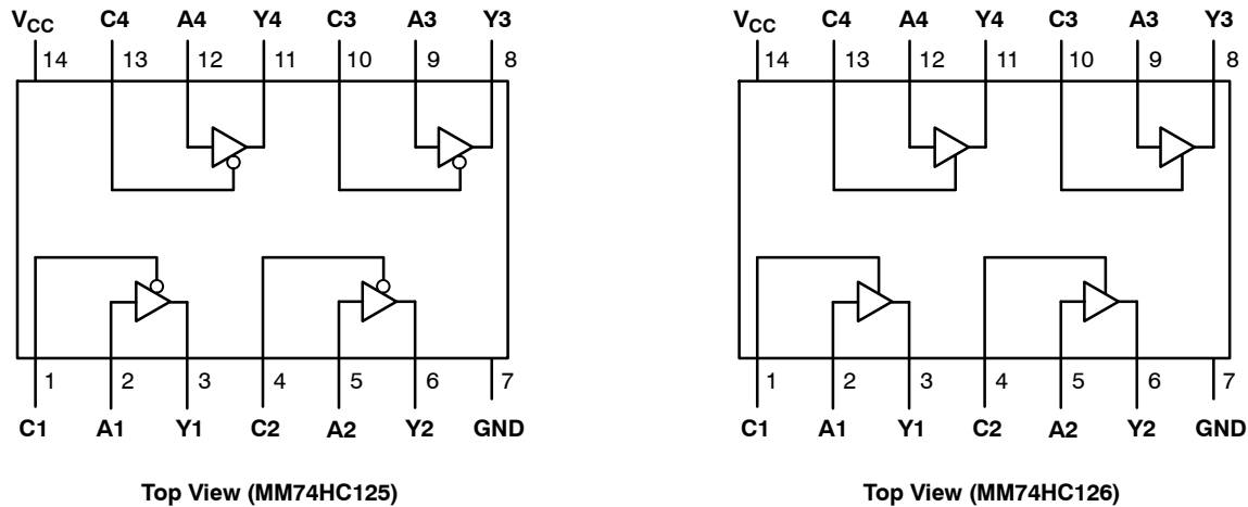
Figure 1. Pin Assignments for SOIC and TSSOP
