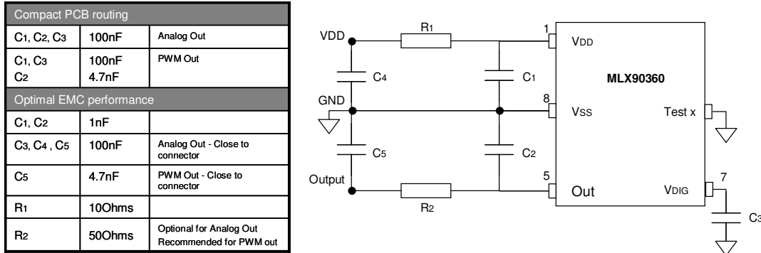
Figure 13 – Recommended wiring for the MLX90360 in SOIC8 package
