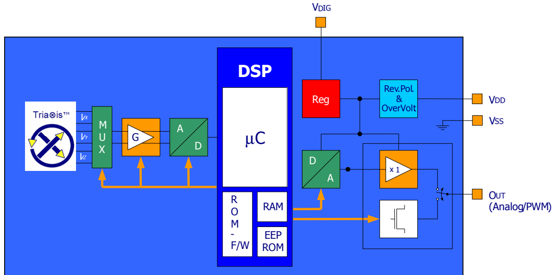
Figure 1 - MLX 90360 Block Diagram
