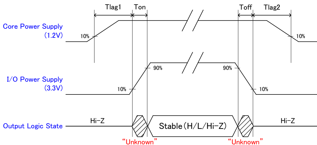
Figure 25: Power Up/Down Sequence - 1
