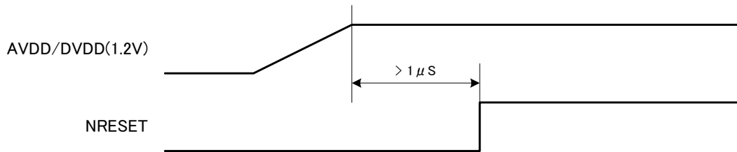
Figure 9: Power-on reset timing chart
