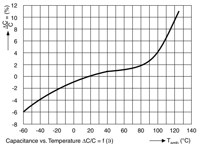
Capacitance vs. Temperature \Delta C/C = f(T) Capacitance as a function of temperature (typical curve)
