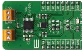
H-Bridge 5 Click
