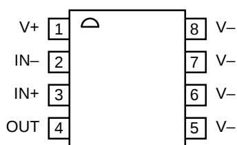
MSOP-8 (MM)
