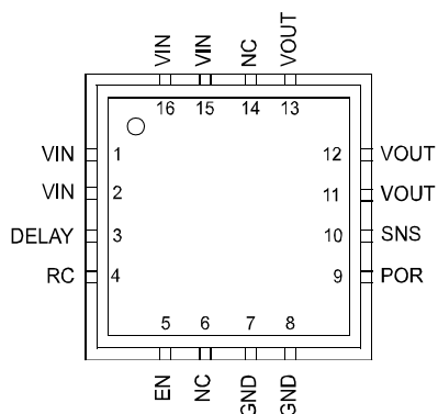
16-Pin 4mm × 4mm MLF® (ML) Fixed Voltages
