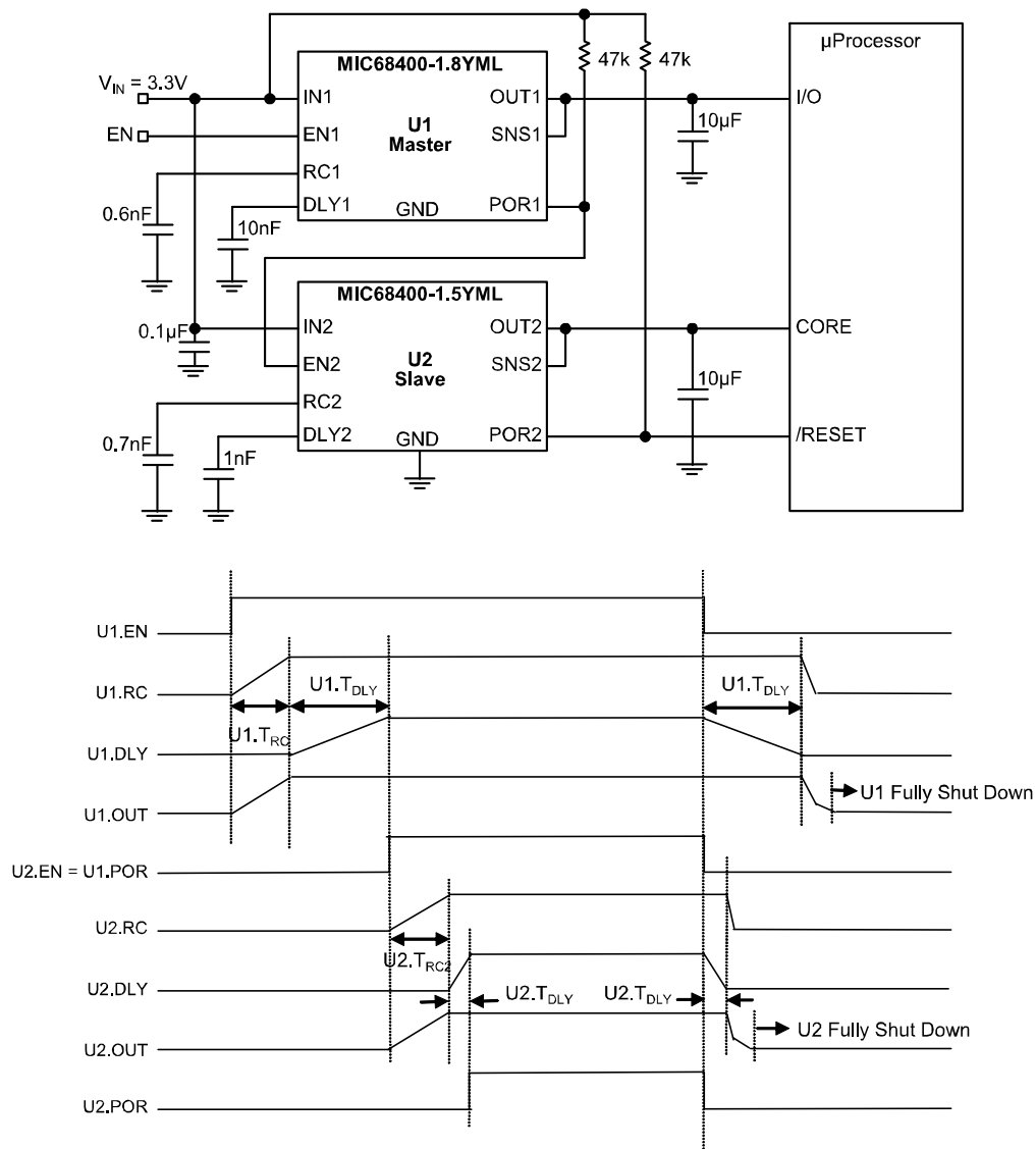
Sequenced Dual Power Supply for I/O and Core Voltage of \mu Processor
