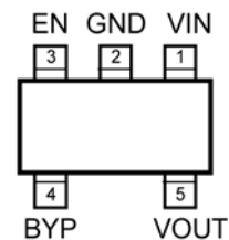
MIC5319 (Adjustable) TSOT-23-5 (D5) Top View
