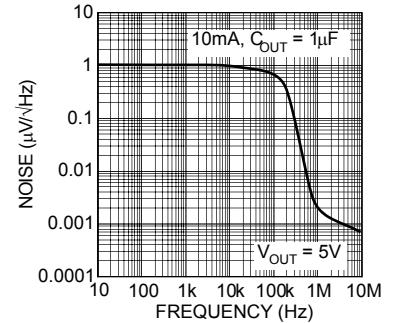
Noise Performance
