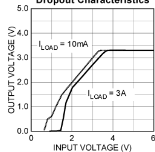
MIC29300-3.3 Dropout Characteristics
