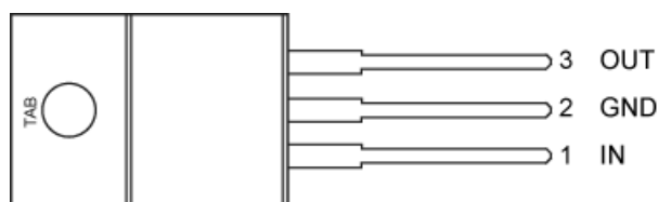
3-Pin TO-220 (T) MIC29150/29300/29500
