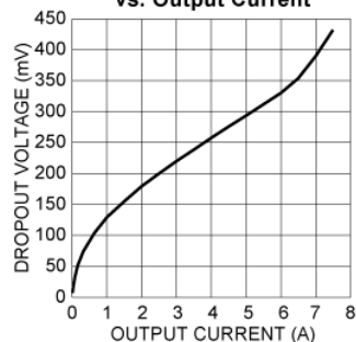
MIC2975x Dropout Voltage vs. Output Current
