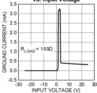
MIC2975x Ground Current vs. Input Voltage
