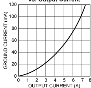
MIC2975x Ground Current vs. Output Current
