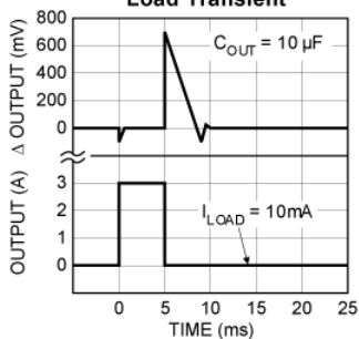
MIC2930x Load Transient
