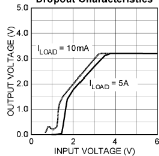
MIC29500-3.3 Dropout Characteristics
