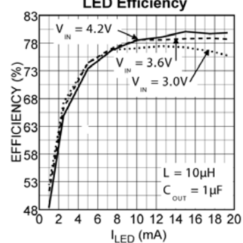
MIC2292 6 Series LED Efficiency
