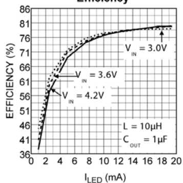
MIC2292 3 Series LED Efficiency
