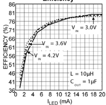
MIC2293 3 Series LED Efficiency
