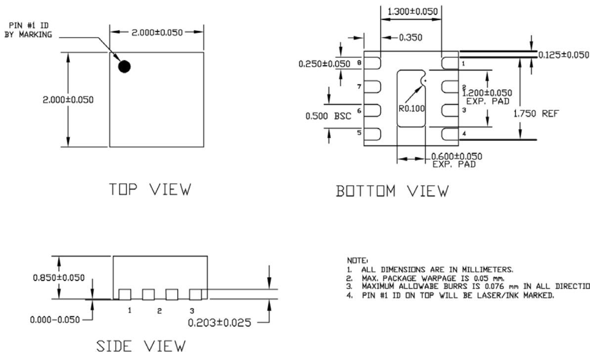
8-Pin MLF ® (ML)
