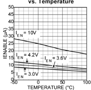
EN Pin Bias Current vs. Temperature
