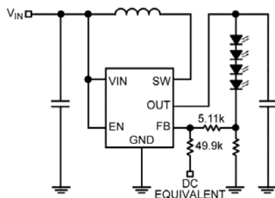
Figure 2. Continuous Dimming
