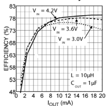
MIC2293 6 Series LED Efficiency
