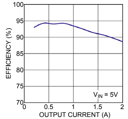
Efficiency VOUT=1.2V
