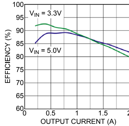
Efficiency VOUT=1.8V
