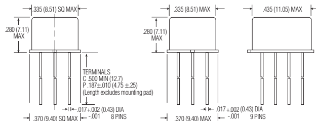
MGA/MGAD/MGADD ENCLOSURE
