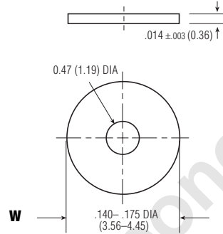
MGA/MGAD/MGADD MOUNTING PAD
