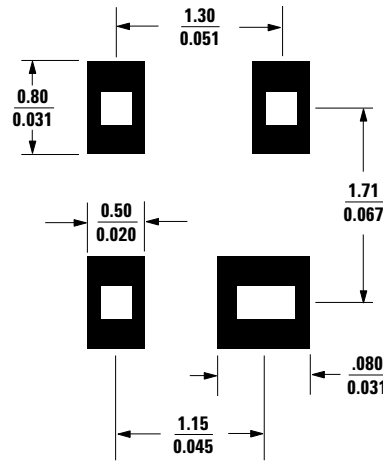
Figure 5. PCB Pad Layout for MGA-53543 Package (dimensions in mm/inches).
