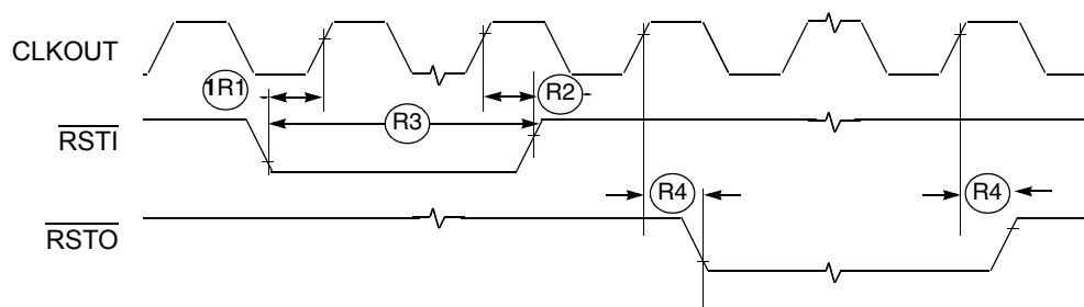
Figure 6. \overline{\text{RSTI}} and Configuration Override Timing
