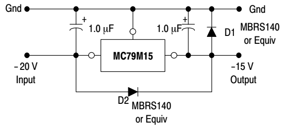
Figure 2. Protection Diodes
