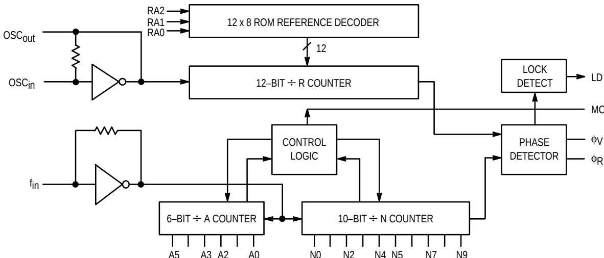
MC145152-2 BLOCK DIAGRAM
